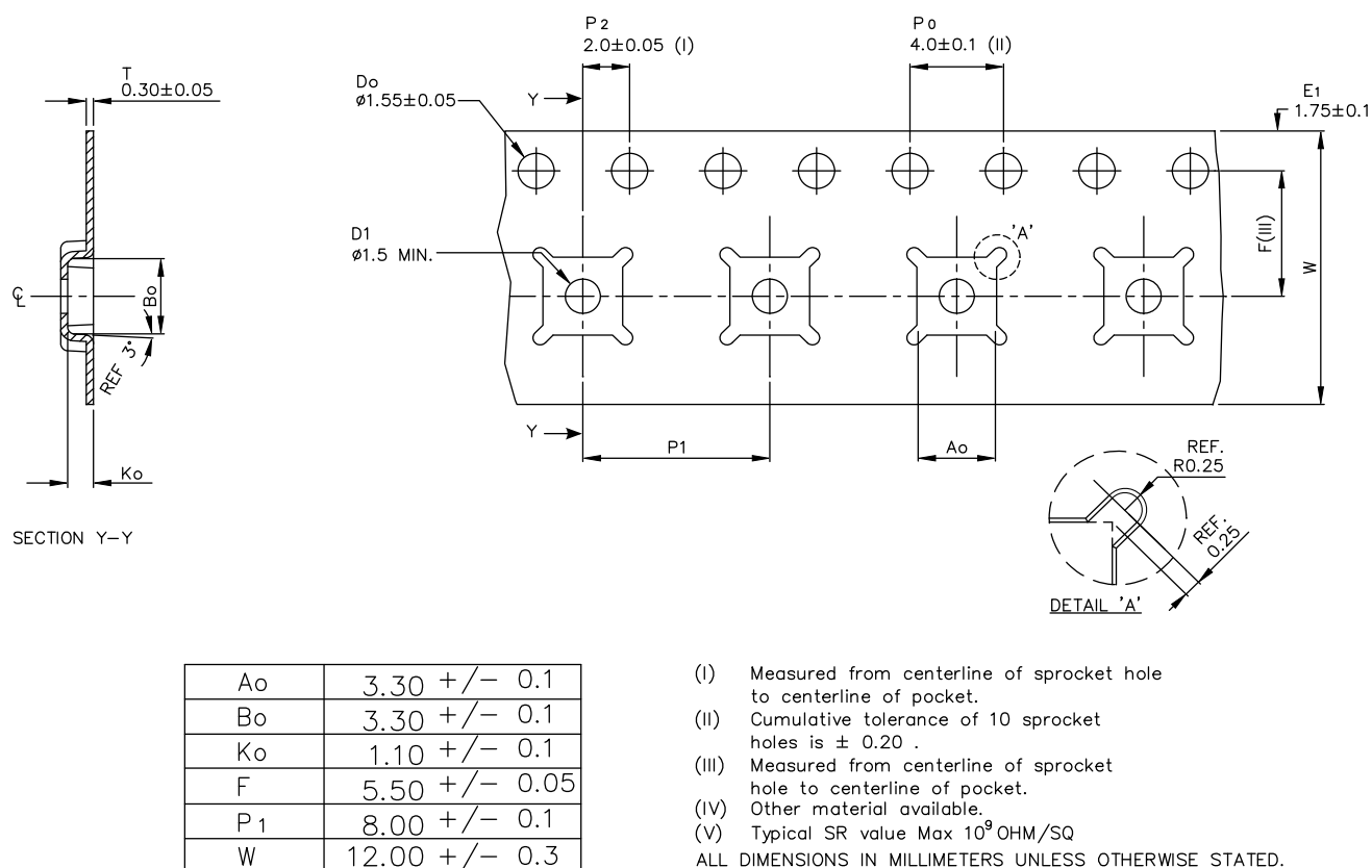
Figure 27. Tape dimensions
