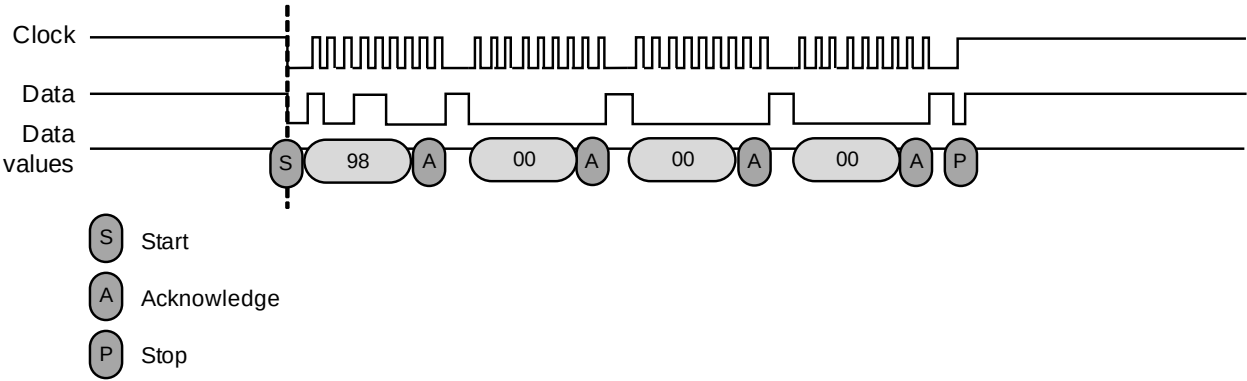
Figure 11. I²C timing diagram
