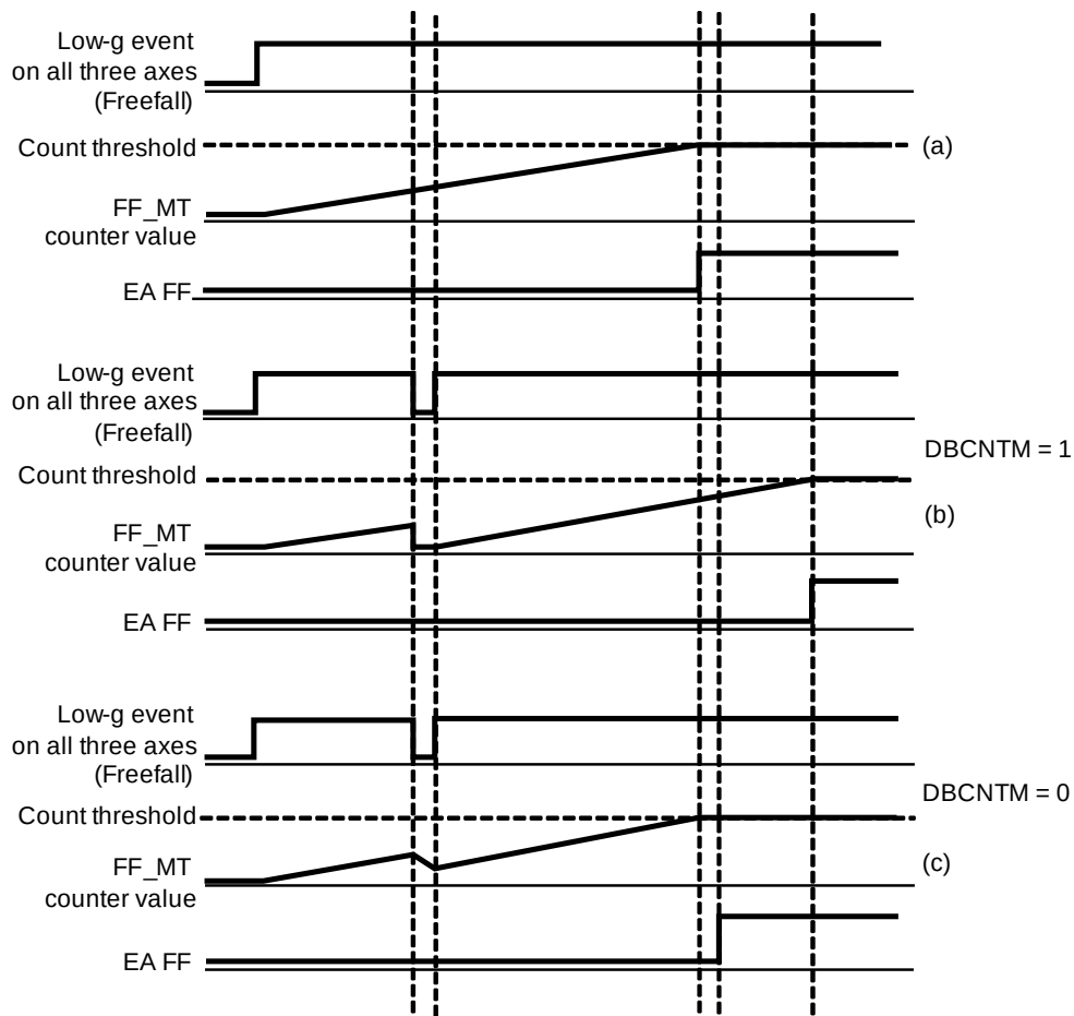
Figure 23. Debounce counter behavior
